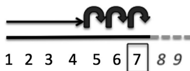
Figure 1. Illustration of a counting procedure for the problem 4 + 3 .
